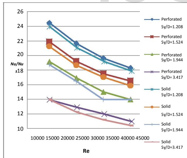
Fig.4. Variation of Nu/Nus based on Projected area with Reynolds No. for various inter-fin spacing at constant C/H = 0
