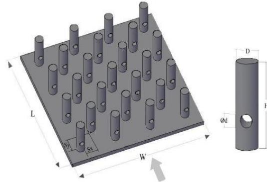
Fig.1. Base Plate with fins in staggered arrangement
