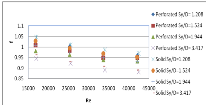
Fig.6. Variation of friction factor with Reynold No. for various inter-fin spacing at C/H=0
