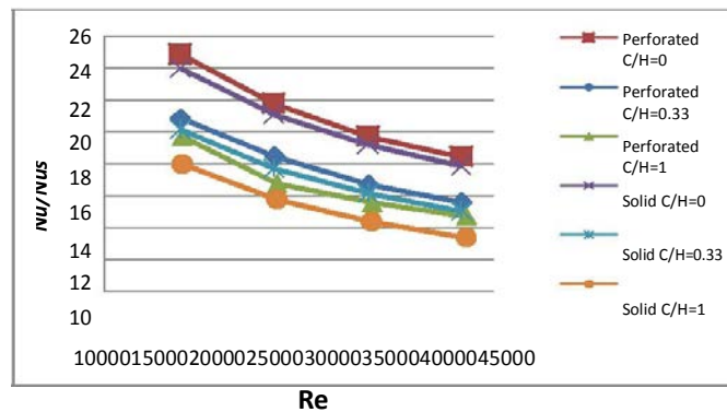
Fig.3. Variation of Nu/Nus based on Projected area with Reynolds No. for various clearance ratio at constant Sy/D=1.208
