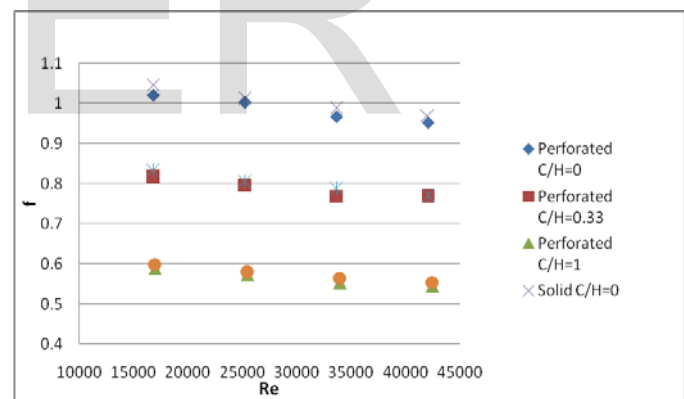
Fig.5. Variation of friction factor with Reynold No. for various clearance ratio at Sy/D=1.208
