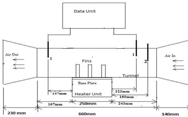
Fig.2 Experimental Set-up (1) RTD Sensor (2) Anemometer
