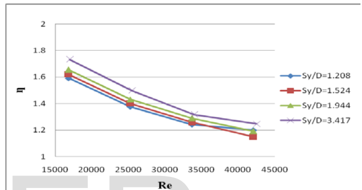
Fig.8. Variation of enhancement efficiency with Reynolds number for various inter-fin spacing ratios at constant C/H = 0.0
