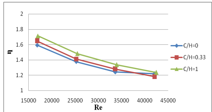
Fig.7 Variation of enhancement efficiency with Reynolds number for various clearance ratios at constant Sy/D = 1.208
